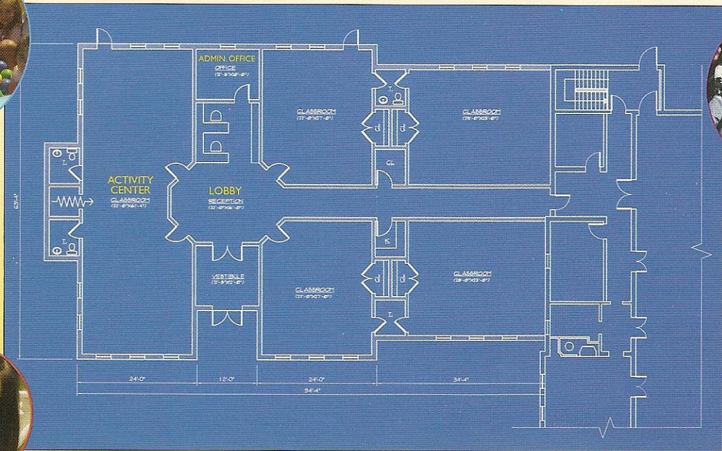
The Martone Children's Center Floor Plan
